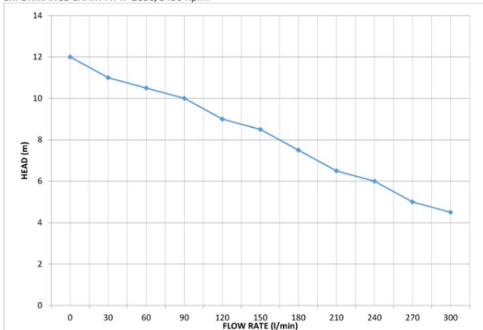
PERFORMANCE CHART AT n=2850/3450 r.p.m
